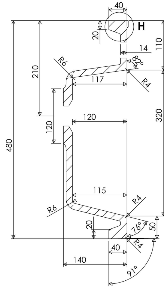
SECTION B-B
