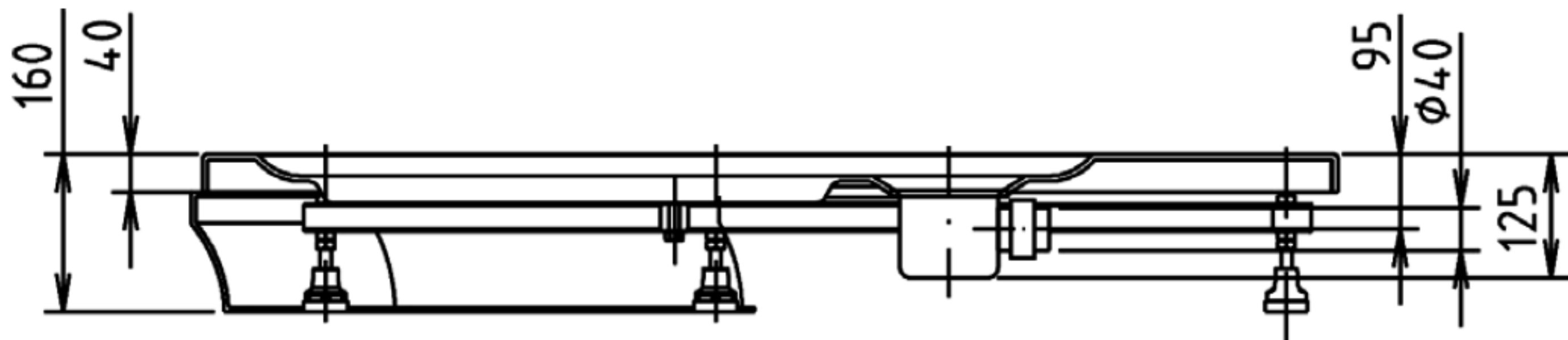
instalace s panelem
