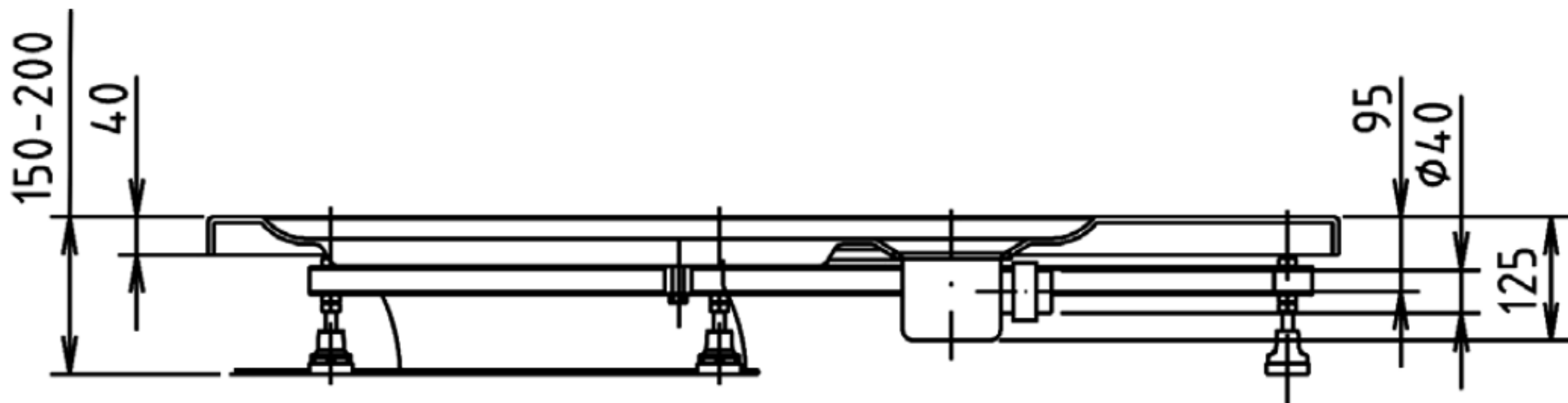
instalace bez panelu
