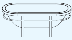
matrix C
