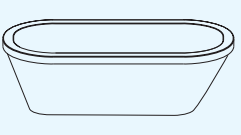
matrix L
